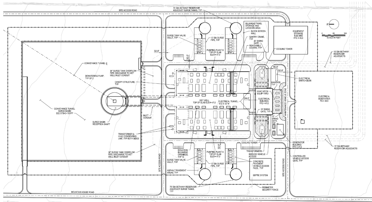
Figure 1. BRPP Facilities Conceptual Configuration and Site Plan
